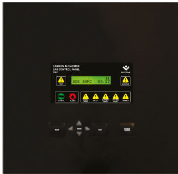
Addressable Carbon Monoxide Control Panel EGPC
